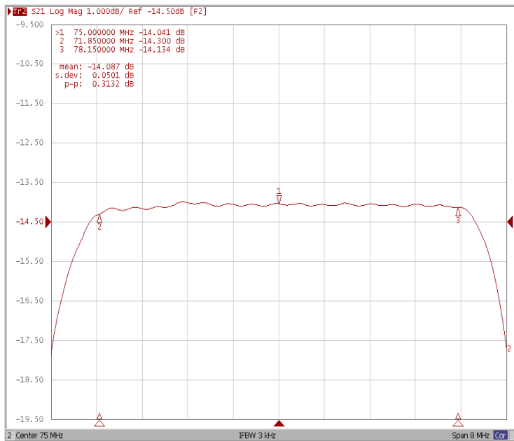
Ripple Variation Fo±3.15MHz
